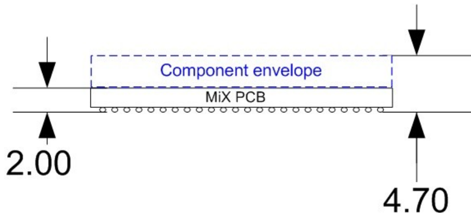
Figure 2 : BLAST height and component envelope
